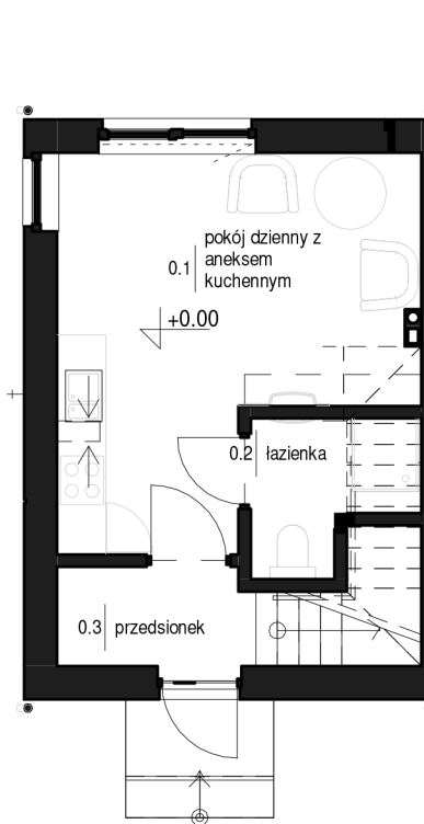
PARTER 1:100
