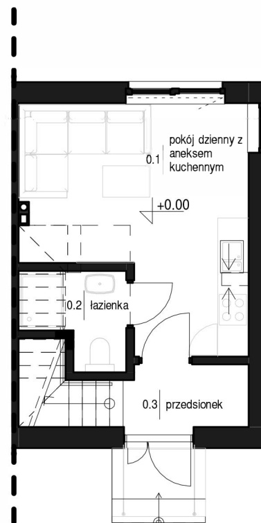
PARTER 1:100
