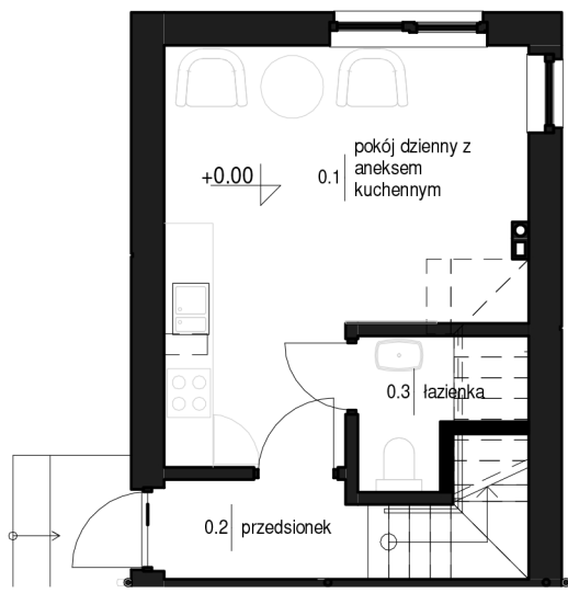
PARTER 1:100
